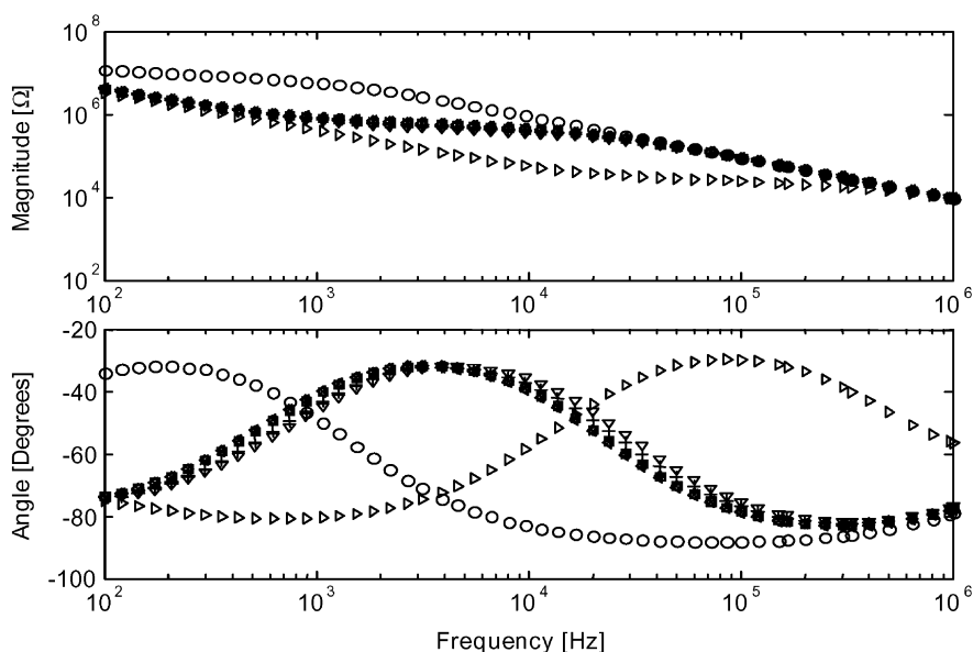
Fig. 7. Complex impedance (magnitude and angle) of DI water (○), Tris–Gly–Dext (◁), and six different samples of L. innocua : 1–4 dead (x) and live (o) cells, 50–200 dead (□) and live (▷) cells, 5000–20,000 dead (+) and live (>) cells. These numbers correspond to the number of cells in the 5.27 nl chamber in the chip, where impedance is measured.
